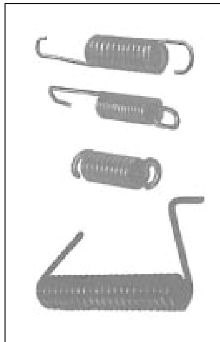
REF. 05151 MUELLE VARIADOR REF. 05207 MUELLE MORDAZA TRASERA REF. 05208 MUELLE MORDAZA DELANTERA, VESPINO GL REF. 05209 MUELLE MORDAZA DELANTERA REF. 05521 MUELLE FARO REF. 05522 MUELLE ZAPATA EM- BRAGUE REF. 05253 MUELLE EMBRAGUE 3 PIEZAS REF. 05401 MUELLE CABALLETE
